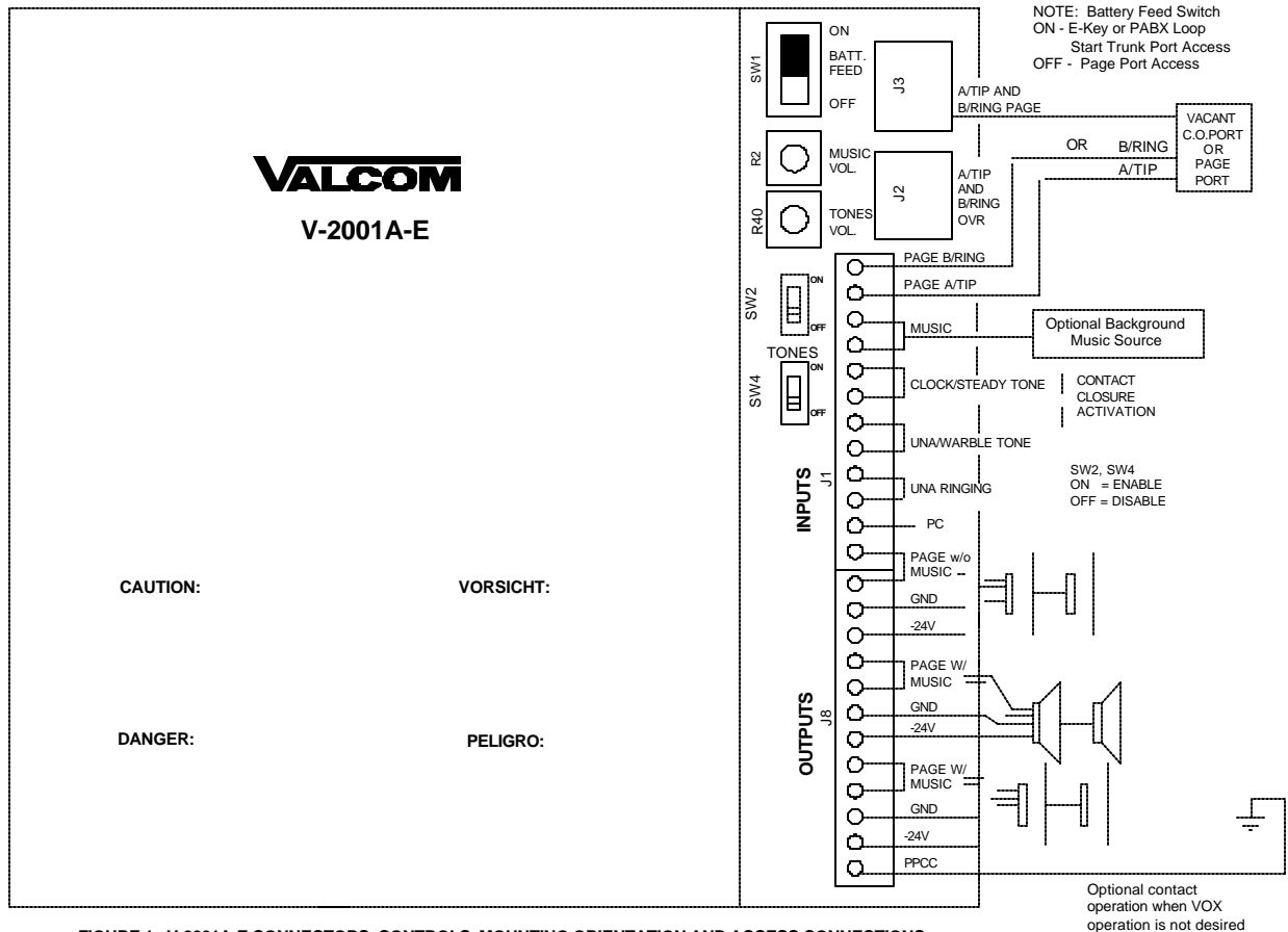
FIGURE 1: V-2001A-E CONNECTORS, CONTROLS, MOUNTING ORIENTATION AND ACCESS CONNECTIONS
