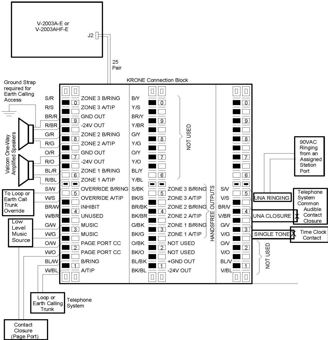
FIGURE 2 - CONNECTIONS FOR THE V-2003A-E AND THE V-2003AHF-E
